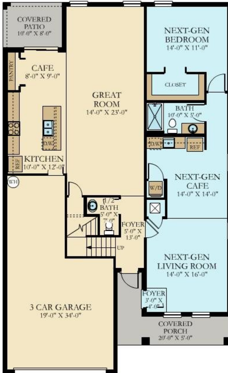
FIRST FLOOR
