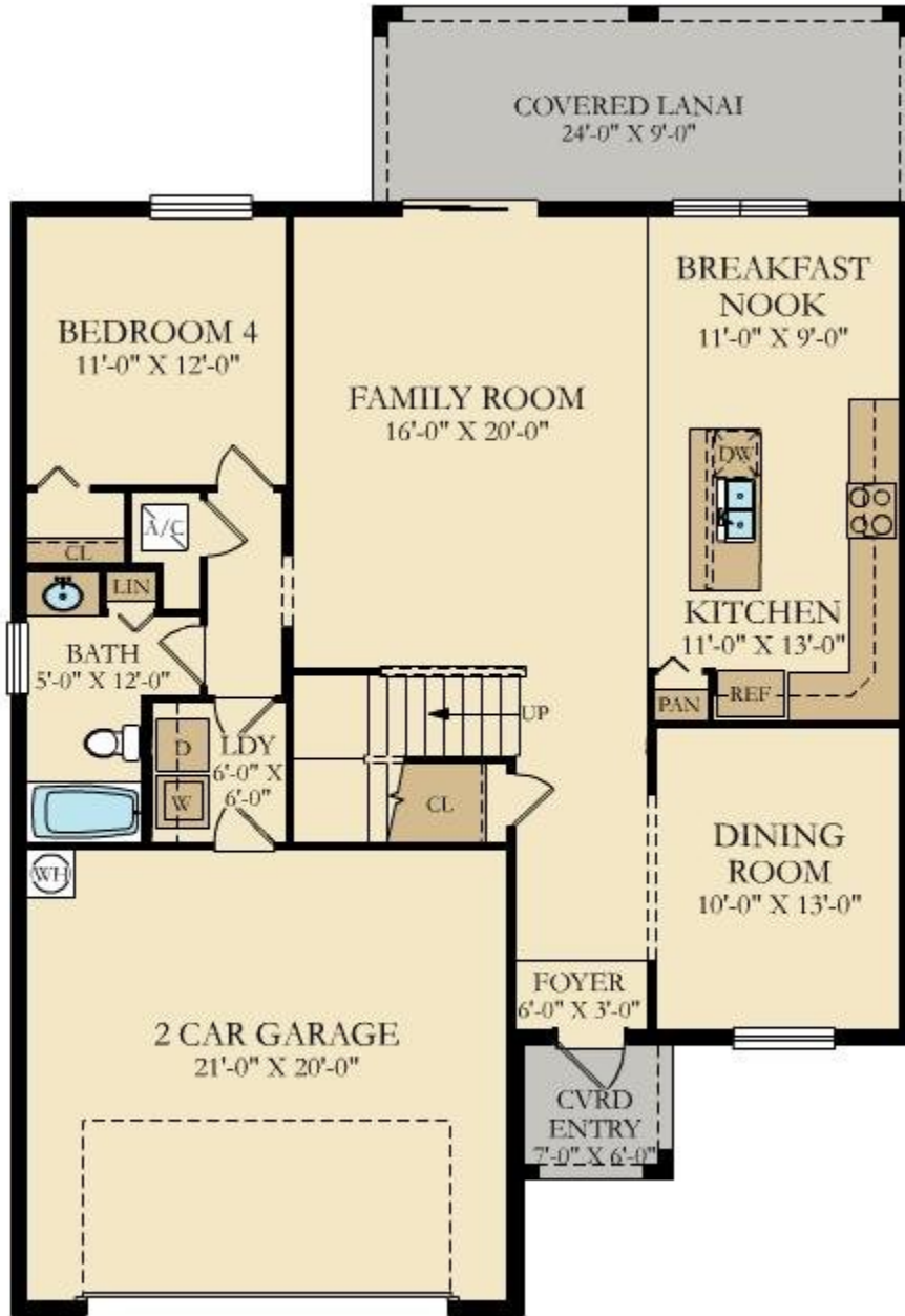
FIRST FLOOR
