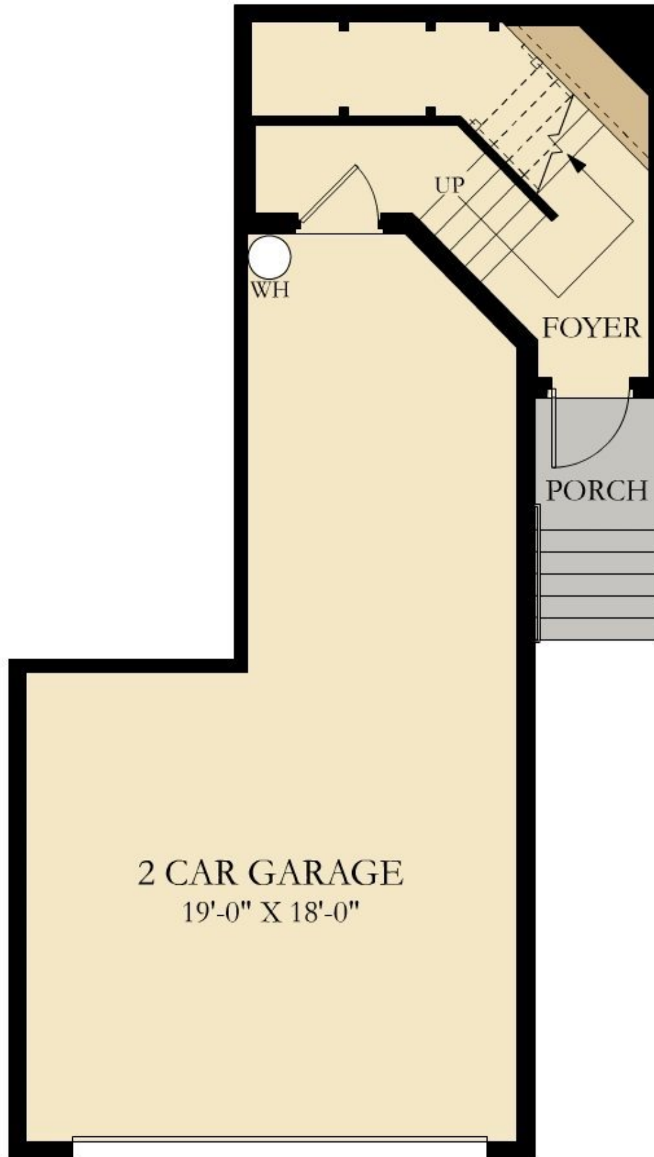
FIRST FLOOR
