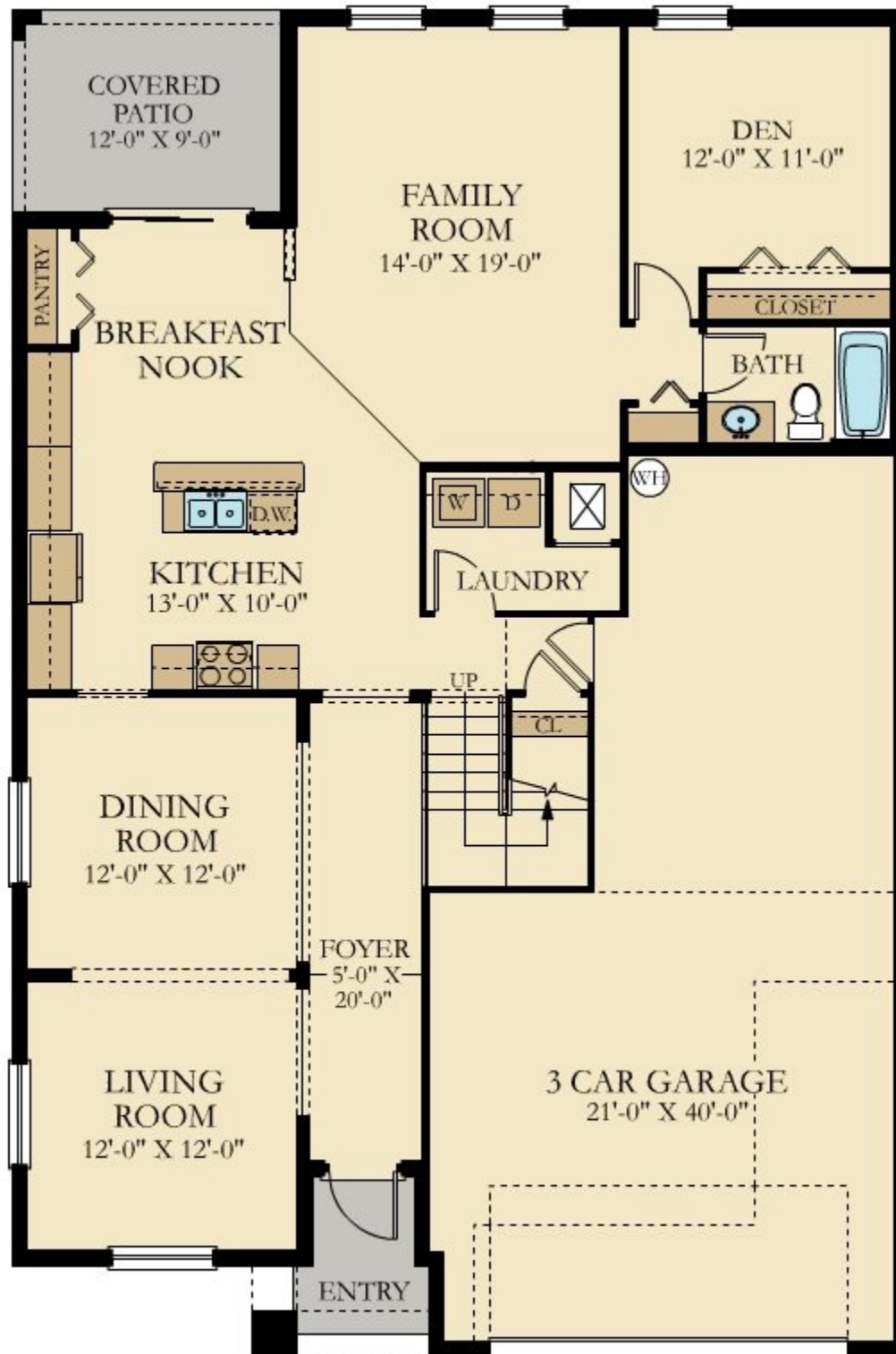
FIRST FLOOR
